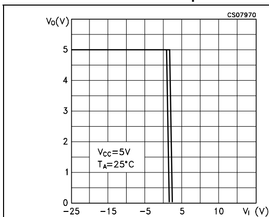
Figure 8. Voltage transfer characteristics for transmitter inputs
